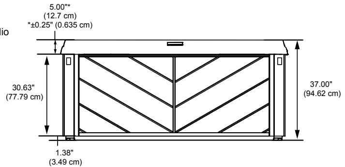
FRONT/BACK VIEW
