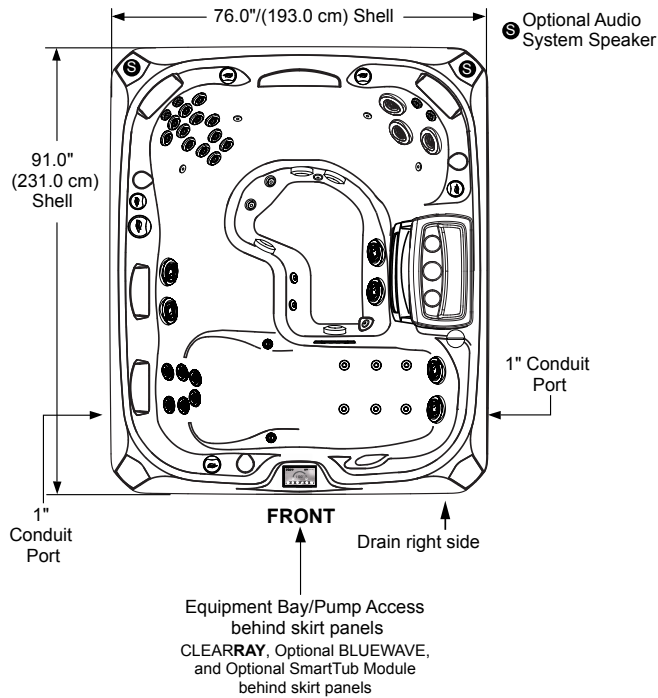
TOP VIEW
