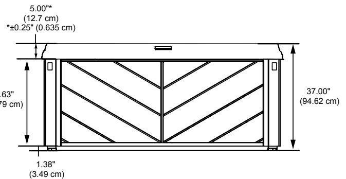
FRONT/BACK VIEW Tolerance: \pm 0.5" (1.27 cm)
