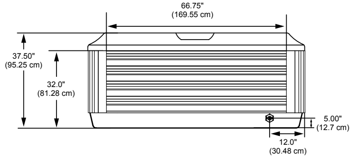
LEFT SIDE VIEW Tolerance: \pm 0.5" (1.27 cm)
